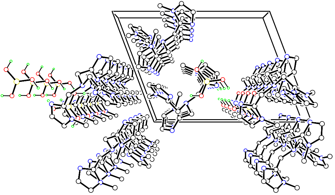
Supplementary Fig. 3. Packing diagram for (I) viewed normal to the ac plane, illustrating the hydrogen-bonding network between tmima and boric acid molecules, and the hydrophobic boundaries.
