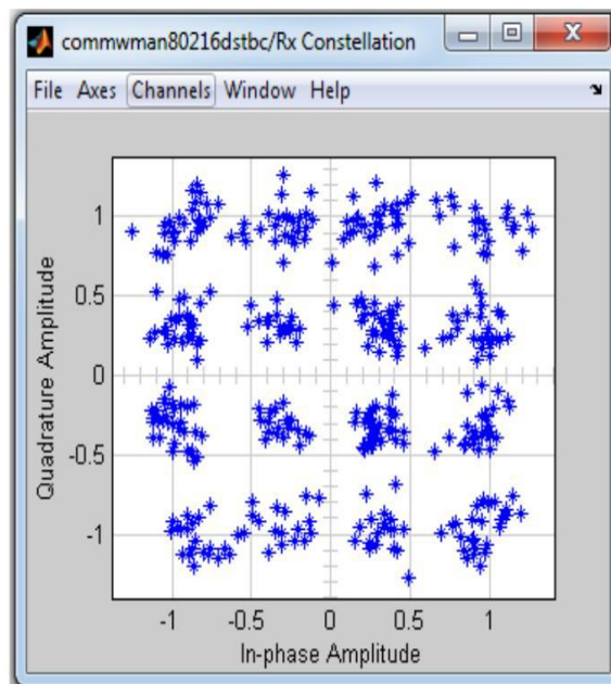
Fig5. Constellation of Receiver Section
